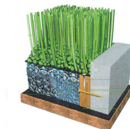
Playground Turf: Looks and feels natural. Impact-absorbing mat provides protection. Concrete subsurface is not required.
