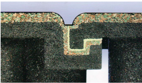
Interlocking Tiles: 2'x2' with various thicknesses in a large number of colors. Requires a concrete subsurface.
